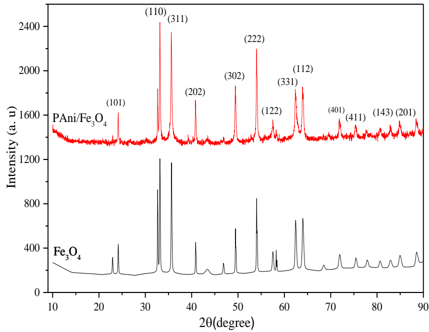
Fig. 5: XRD analysis of modified Fe 3 O 4 nanoparticles and PAni/Fe 3 O 4 nanocomposites
