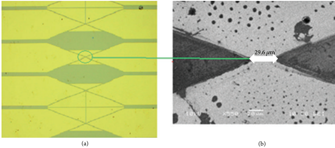
FIGURE 4: (a) The HPM image of gold electrodes. (b) An enlarged SEM image of the fabricated gold electrodes.
