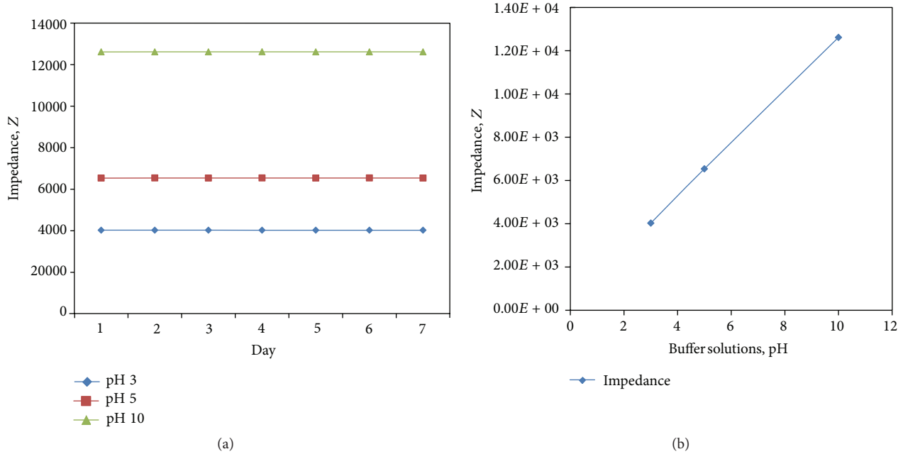
FIGURE 9: Impedance variation of one sensor in pH buffer solutions in seven consecutive days.
