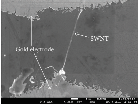
FIGURE 6: FESEM result of individual SWNT aligned at 5 V peak-to-peak and 20 MHz in dielectrophoresis process.
