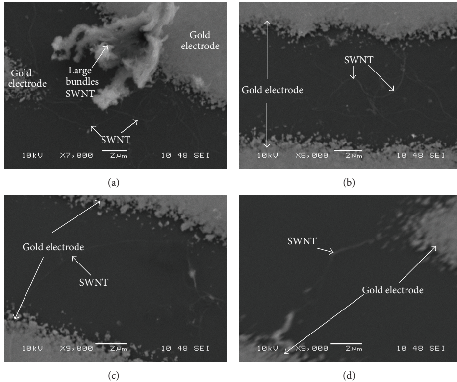
FIGURE 5: SEM images of SWNTs' alignment. (a) 1 V, 10 MHz. (b) 1 V, 20 MHz. (c) 5 V, 10 MHz. (d) 5 V, 20 MHz.
