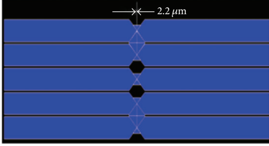
FIGURE 1: Schematic structure of the teeth-like electrode design.
