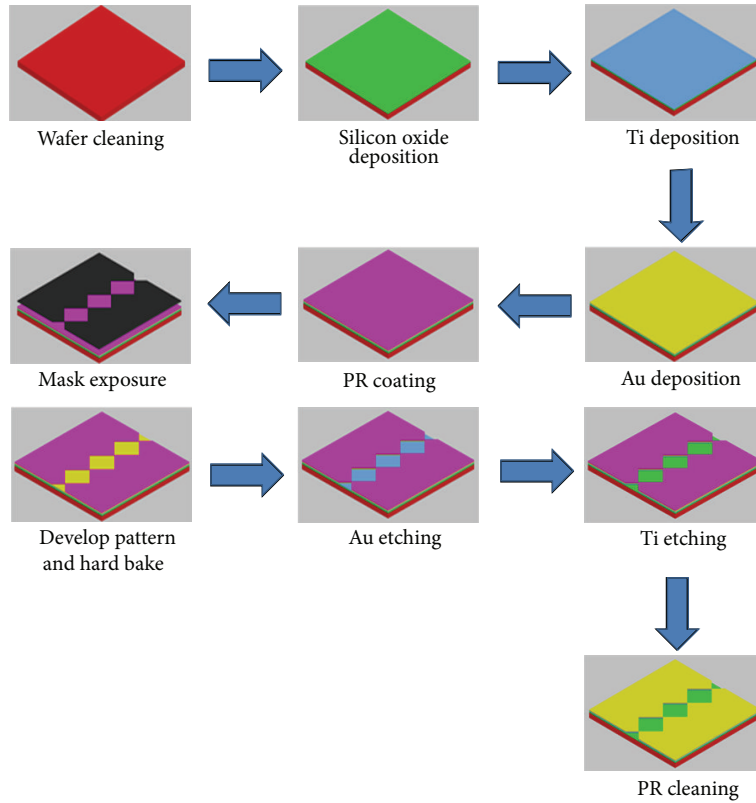
FIGURE 2: Fabrication process of the gold electrodes.
