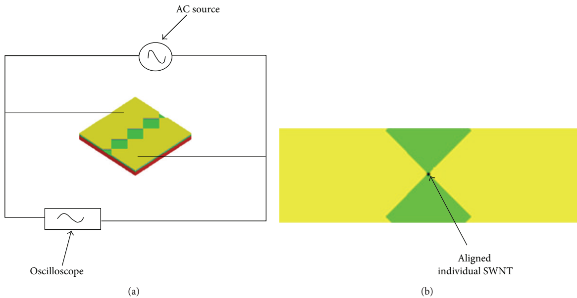
FIGURE 3: (a) Experimental setup for dielectrophoresis of the CNTs. (b) Schematic diagram of the SWNT alignment.
