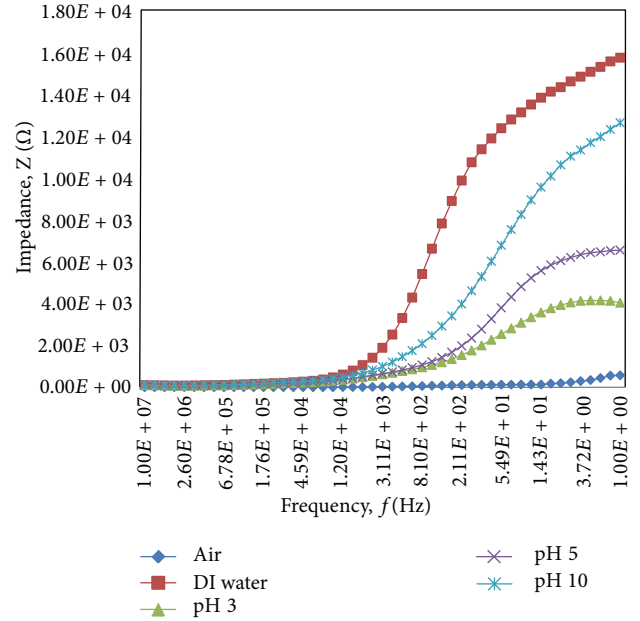
FIGURE 8: Impedance-frequency plot for after SWNT is aligned.
