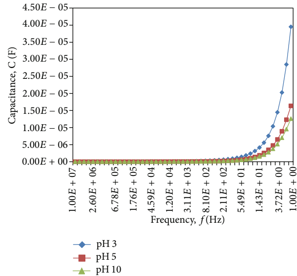
FIGURE 10: Capacitance variation of pH 3, pH 5, and pH 10 without alignment of SWNT.
