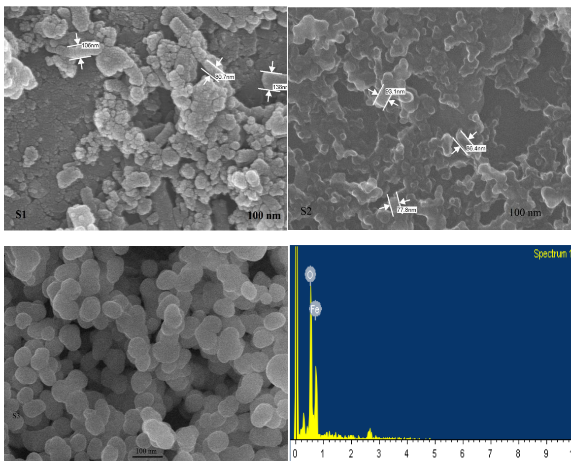
Figure 5. FESEM image of magnetite nanoparticles annealed under vacuum at 200^\circ\text{C} for S1, 300^\circ\text{C} for S2 and 400^\circ\text{C} for S3 and the EDS image of magnetite ( \text{Fe}_3\text{O}_4 ) nanoparticles.
