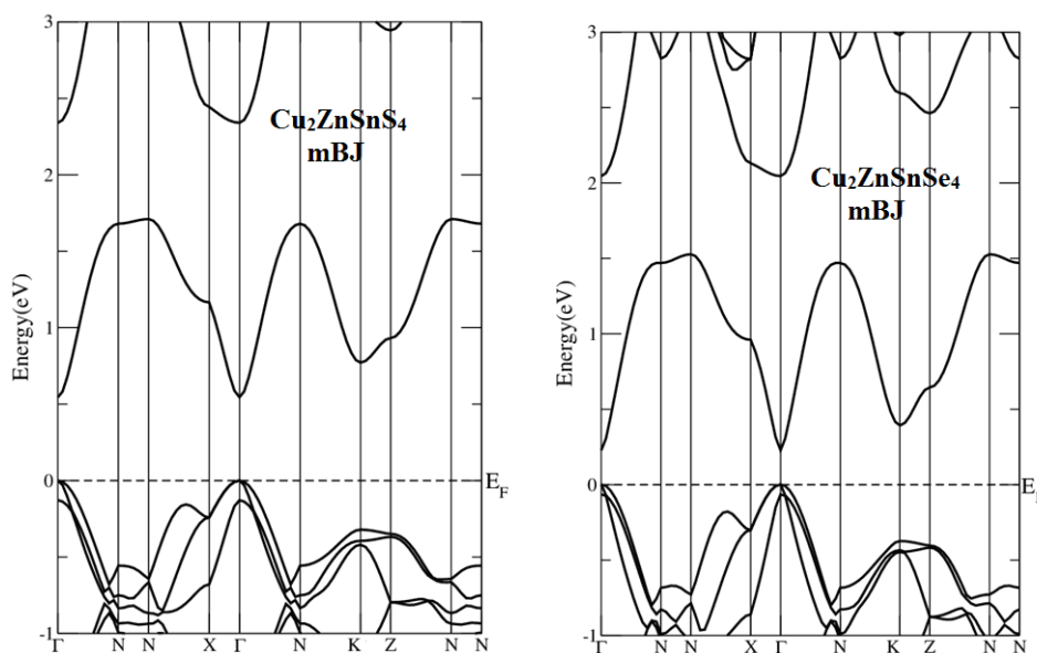
Figure 2. Calculated band structure using mBJ.
