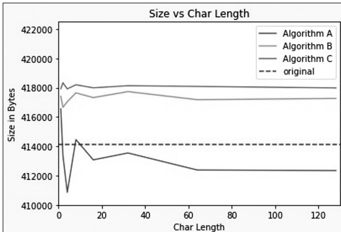
Figure 4: File Size vs Embedded Characters Length
