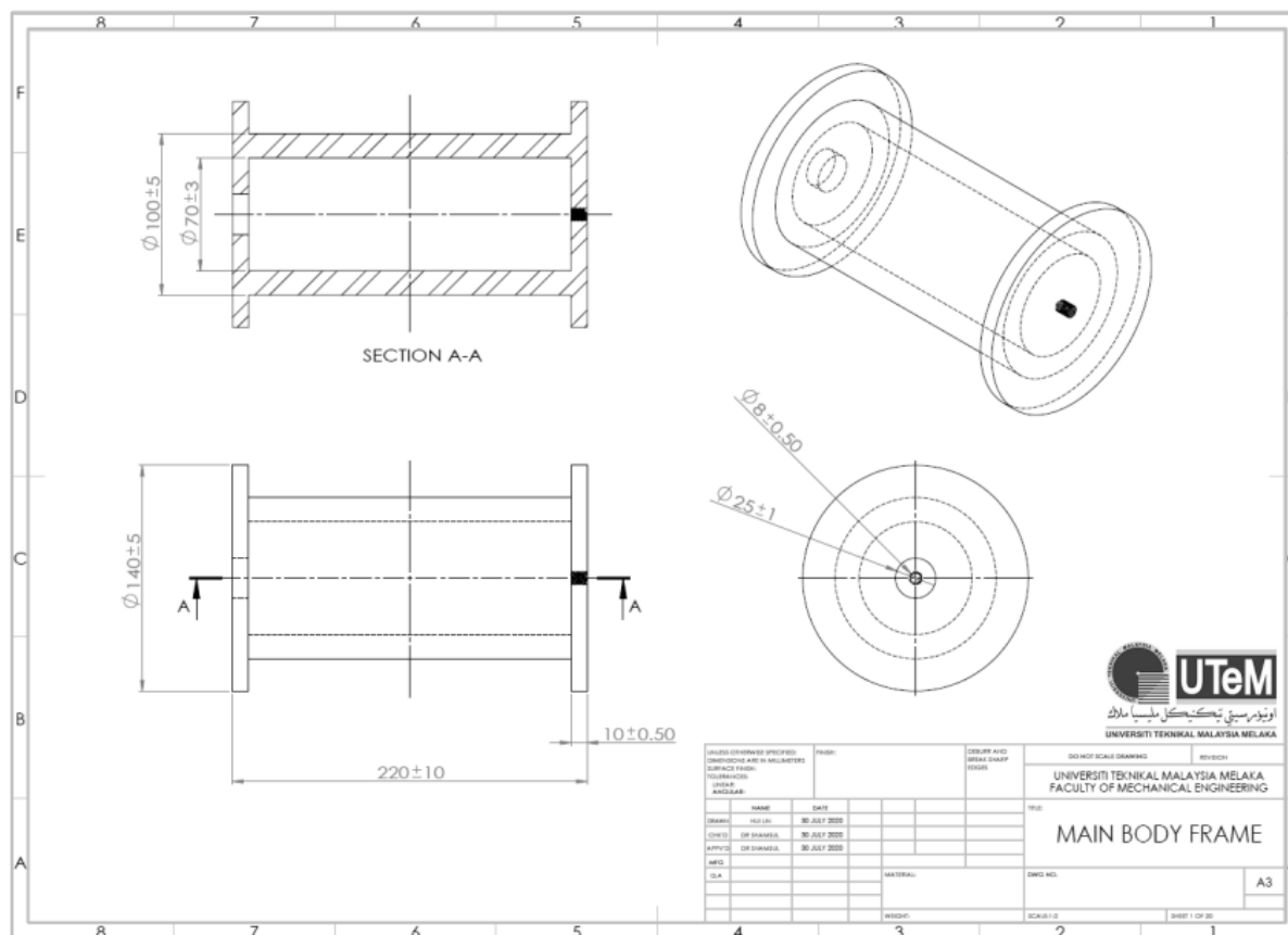
Figure 9. The dimensions in millimeters of the main body frame (roller) in multiple views.
