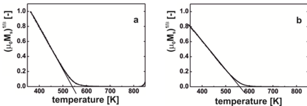
Figure 4. Dependence \mu_0 M_s^{1/3}(T) for alloys: a) \text{Fe}_{50}\text{Co}_{20}\text{B}_{20}\text{Cu}_1\text{Nb}_9 , b) \text{Fe}_{45}\text{Co}_{25}\text{B}_{20}\text{Cu}_1\text{Nb}_9 .
