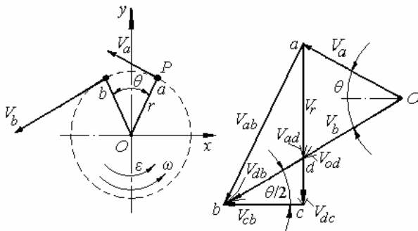
Figure 1. Acceleration of a rotating point.
