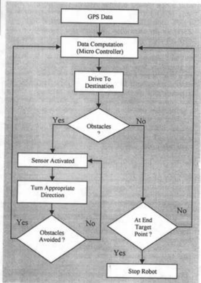
Figure 7 - Software Flowchart For Controller.
