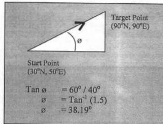
Figure 4 – Trigonometric functions.
