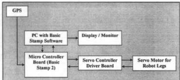
Figure 1 – Block Diagram
