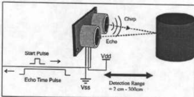
Figure 6 – Ultrasonic Sensor
