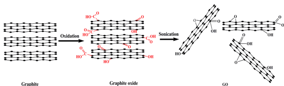
Figure 1. Oxidation of graphite to graphene oxide nanosheets [8].
