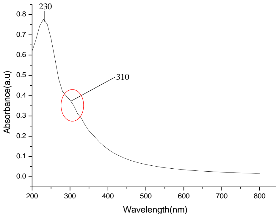
Figure 4. UV-VIS absorbance response of GO dispersion in distilled water after sonication of 1 hour through bath sonication.
