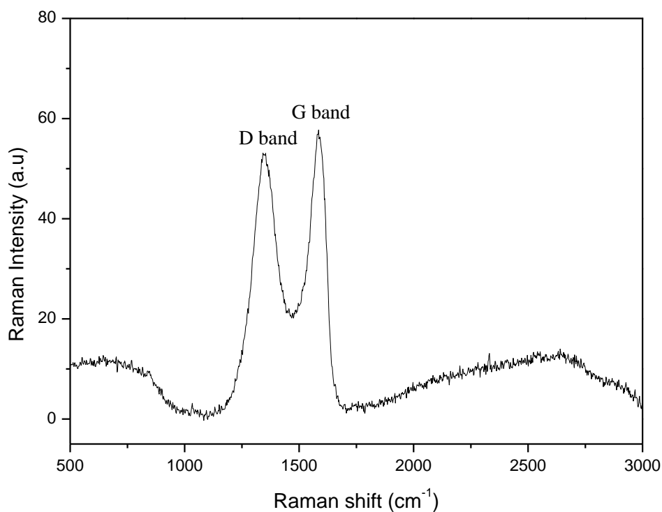
Figure 7. Raman spectra of GO powder.
