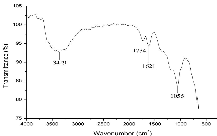
Figure 3. FTIR spectroscopy of GO nanosheets after dried in the oven overnight.
