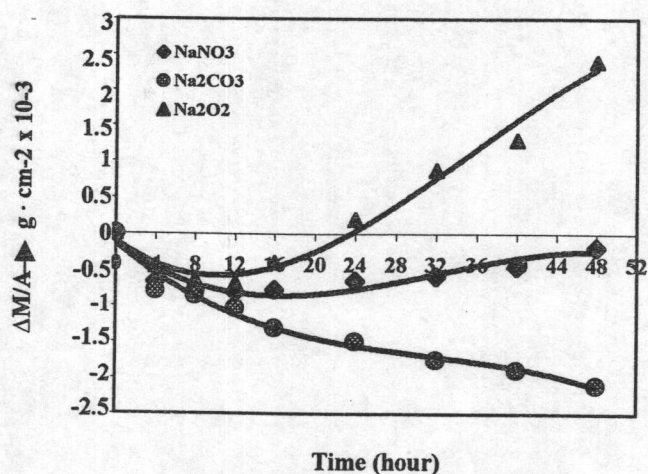
Fig. 1: Oxidation kinetics (mass change versus time) of Nimonic-115 alloy coated with \text{NaNO}_3 , \text{Na}_2\text{CO}_3 & \text{Na}_2\text{O}_2 , oxidized at 850^\circ\text{C} for 48 h.
