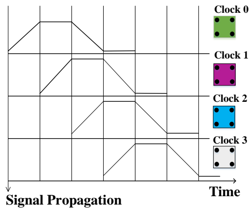
Figure 3. QCA Clocking mechanism.
