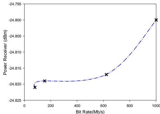
Figure7: Data rate effect on the power receiver.
