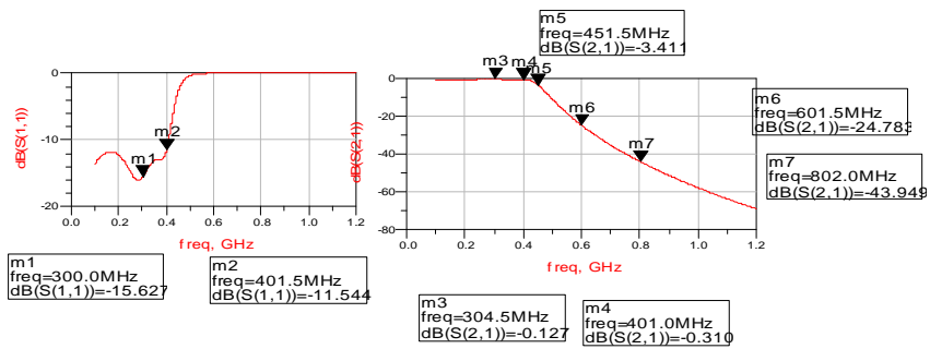
Fig 5. Actual simulation S-parameter result before tuning
