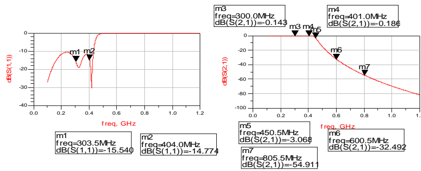
Fig 6. Simulation S-parameter result after tuning
