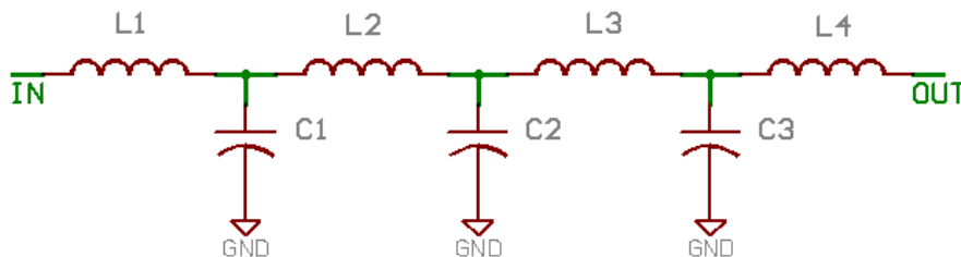
Fig 2. The 7 poles circuit design by filter calculator
