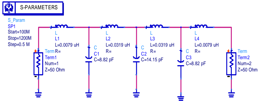
Fig 3. Butterworth low pass filter before tuning cutoff at 450MHz
