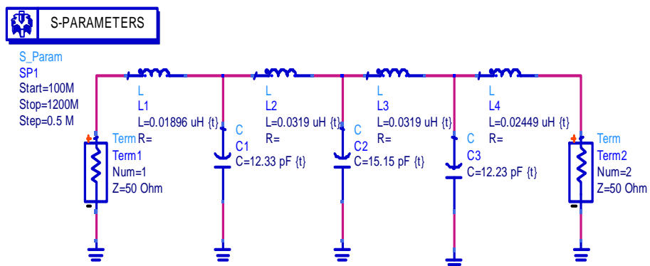
Fig 4. Butterworth low pass filter after tuning cutoff at 450MHz
