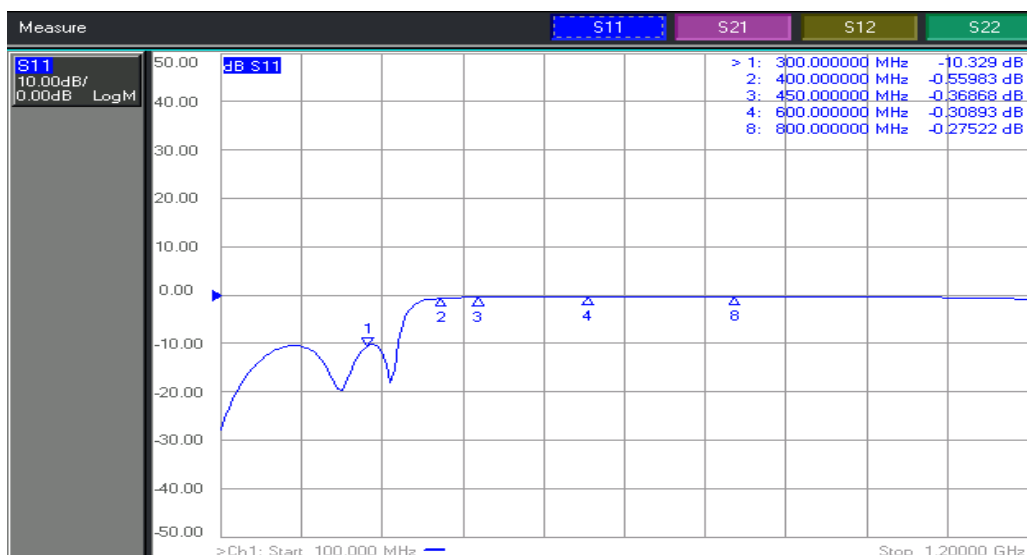
Fig 7. Simulation S11 results for Butterworth low pass filter
