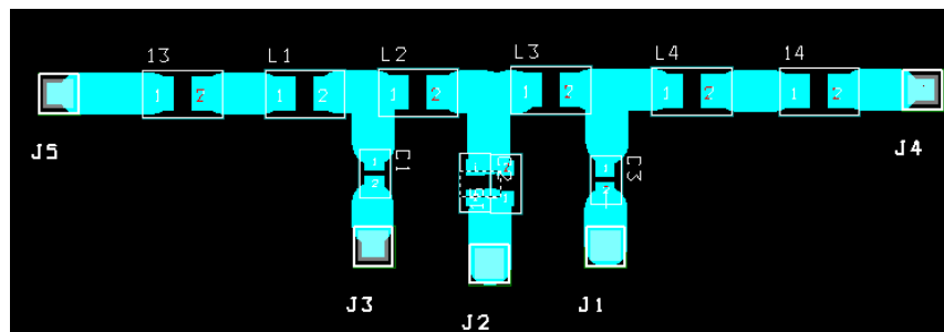
Fig 9. The layout of Butterworth filter design by using orcad
