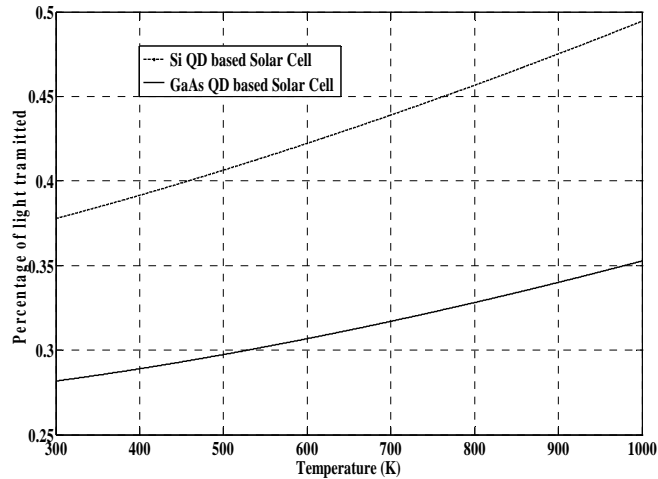
Fig. 2 Effect of temperature on the percentage of light transmitted through the solar cell. The solid line and the dashed line represent the percentage of light transmitted through quantum dot based solar cell using GaAs and Si respectively.
