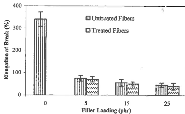
Figure 3: Effect of filler loading on the elongation at break of the LDPE/WHF composites with untreated and treated water hyacinth fibers.
