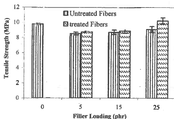
Figure 1: Effect of filler loading on the tensile strength of the LDPE/WHF composites with untreated and treated water hyacinth fibers.
