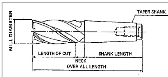
Figure 2: Taper Shank End Mill
