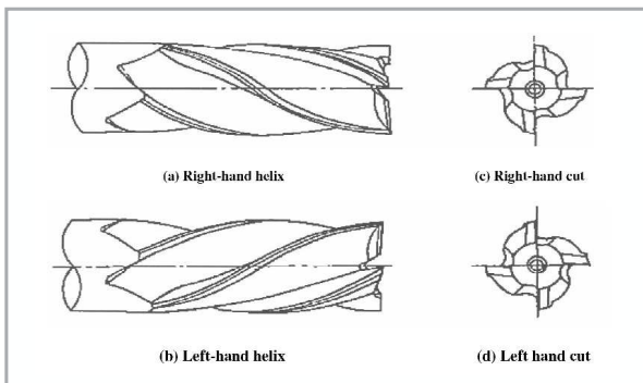
Figure 4: Helix of End Mill
