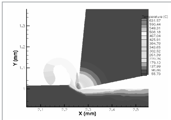
Figure 8: FEM analysis of heat generated during material cutting
