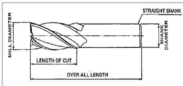
Figure 1: Straight Shank End Mill
