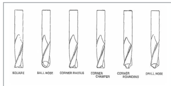
Figure 6: Various types of end profile in end mills
