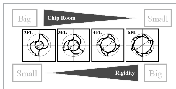
Figure 5: Chip Room and Rigidity of End Mills
