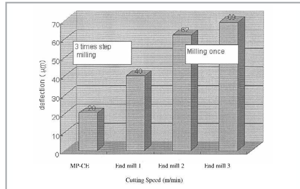
Figure 16: Comparison of the deflection
