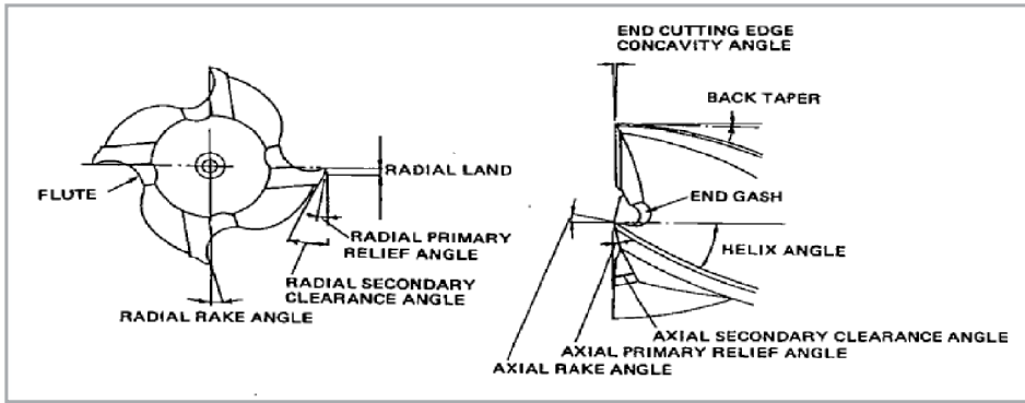
Figure 3: Terminology of an End Mill
