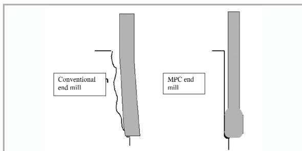
Figure 12: Comparison between MPC and conventional end mills
