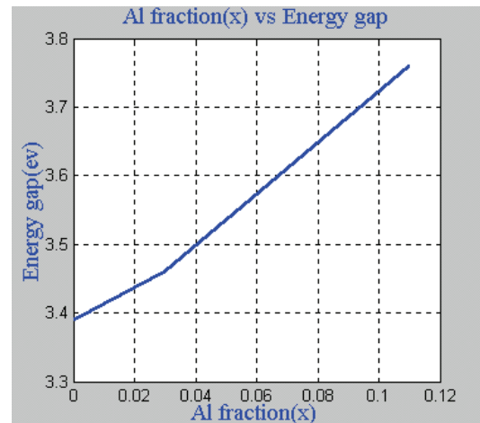
Figure 6. Dependence of band gap on photon Al fraction (x) for \text{Al}_x\text{Ga}_{1-x}\text{N}
