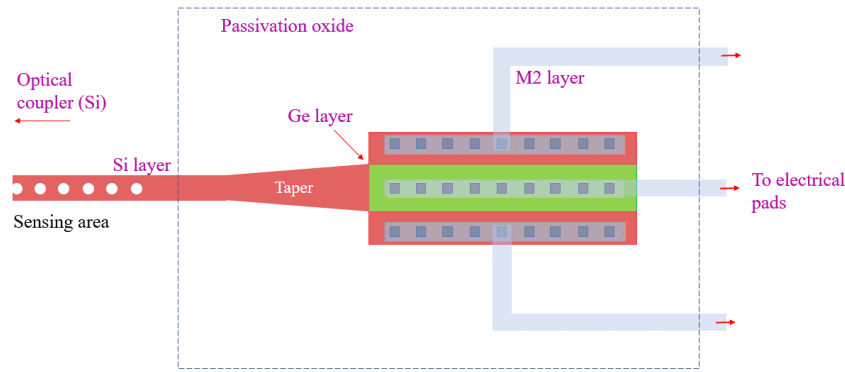
Figure 14. The illustration of the GDS layout design (not to scale) without the doping layers, following the generic silicon photonics (GSiP) technology design rules and layers arrangement.
