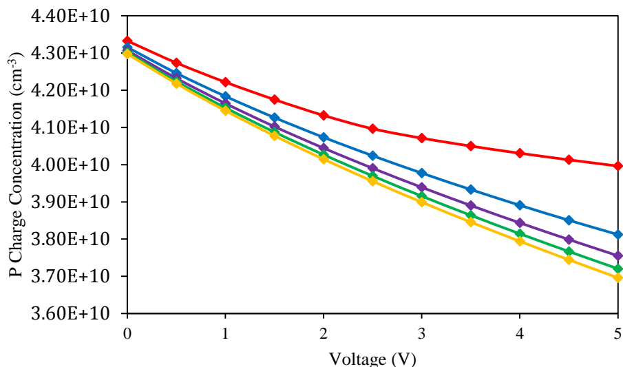
Figure 15. P charge concentration for different N dopant concentration in the waveguide. (Red line: N carrier doped at 0.5 \times 10^{17} \text{ cm}^{-3} ; Blue line: N carrier doped at 1.0 \times 10^{17} \text{ cm}^{-3} ; Purple line: N carrier doped at 1.5 \times 10^{17} \text{ cm}^{-3} ; Green line: N carrier doped at 2.0 \times 10^{17} \text{ cm}^{-3} ; Yellow line: N carrier doped at 2.5 \times 10^{17} \text{ cm}^{-3} ).
