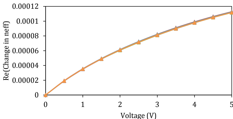
Figure 12. Change in effective index versus voltage applied. (Dark blue line: 200nm waveguide height; Orange line: 220nm waveguide height; Grey line: 240nm waveguide height; Yellow line: 260nm waveguide height; Light blue line: 280nm waveguide height; Green line: 300nm waveguide height).
