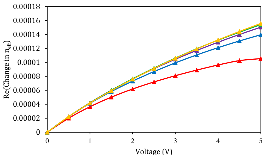
Figure 19. Change in effective index versus voltage applied. (Red line: P carrier doped at 1 \times 10^{17} \text{ cm}^{-3} ; Blue line: P carrier doped at 2 \times 10^{17} \text{ cm}^{-3} ; Purple line: P carrier doped at 3 \times 10^{17} \text{ cm}^{-3} ; Green line: P carrier doped at 4 \times 10^{17} \text{ cm}^{-3} ; Yellow line: P carrier doped at 5 \times 10^{17} \text{ cm}^{-3} ).
