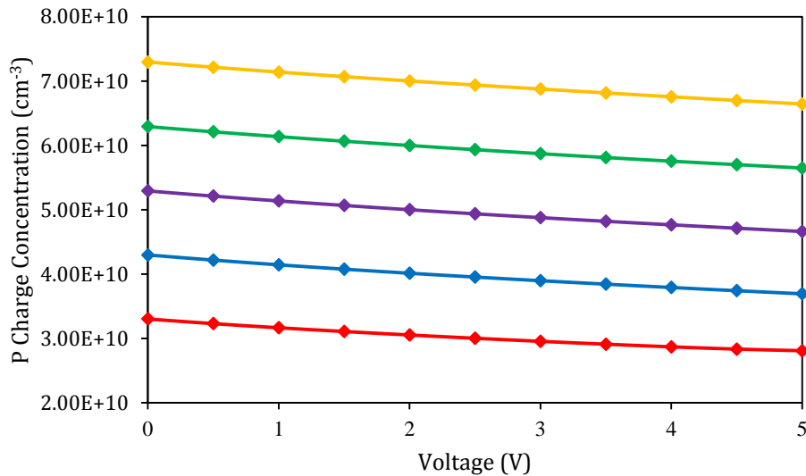
Figure 18. P charge concentration for different P dopant concentration in the waveguide. (Red line: P carrier doped at 1 \times 10^{17} \text{ cm}^{-3} ; Blue line: P carrier doped at 2 \times 10^{17} \text{ cm}^{-3} ; Purple line: P carrier doped at 3 \times 10^{17} \text{ cm}^{-3} ; Green line: P carrier doped at 4 \times 10^{17} \text{ cm}^{-3} ; Yellow line: P carrier doped at 5 \times 10^{17} \text{ cm}^{-3} ).
