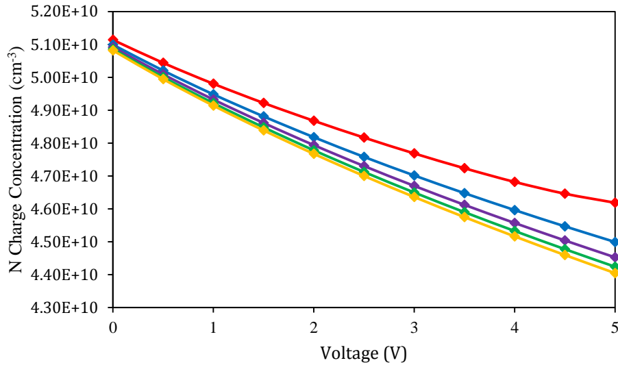
Figure 17. N charge concentration for different P dopant concentration in the waveguide. (Red line: P carrier doped at 1 \times 10^{17} \text{ cm}^{-3} ; Blue line: P carrier doped at 2 \times 10^{17} \text{ cm}^{-3} ; Purple line: P carrier doped at 3 \times 10^{17} \text{ cm}^{-3} ; Green line: P carrier doped at 4 \times 10^{17} \text{ cm}^{-3} ; Yellow line: P carrier doped at 5 \times 10^{17} \text{ cm}^{-3} ).
