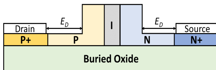
Figure 20. Electrical contacts distance change.
