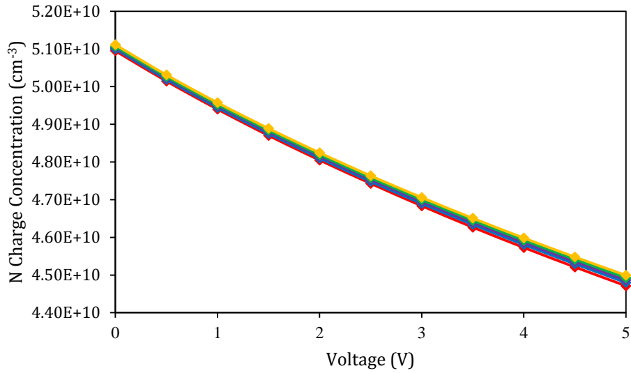
Figure 21. N charge concentration for different electrical contacts distance to the waveguide core. (Red line: E_D = 500nm ; Blue line: E_D = 400nm ; Purple line: E_D = 300nm ; Green line: E_D = 200nm ; Yellow line: E_D = 100nm ).
