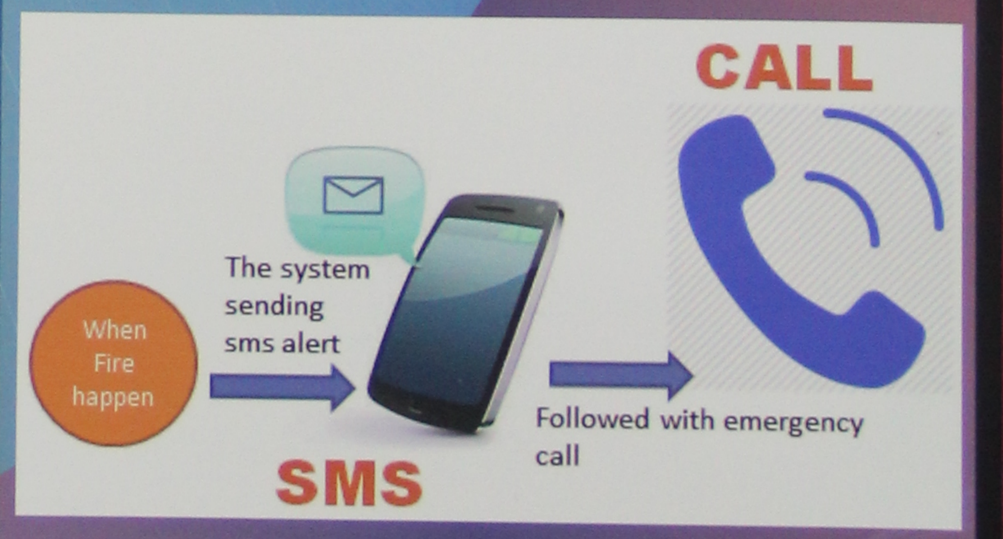
Notification system
