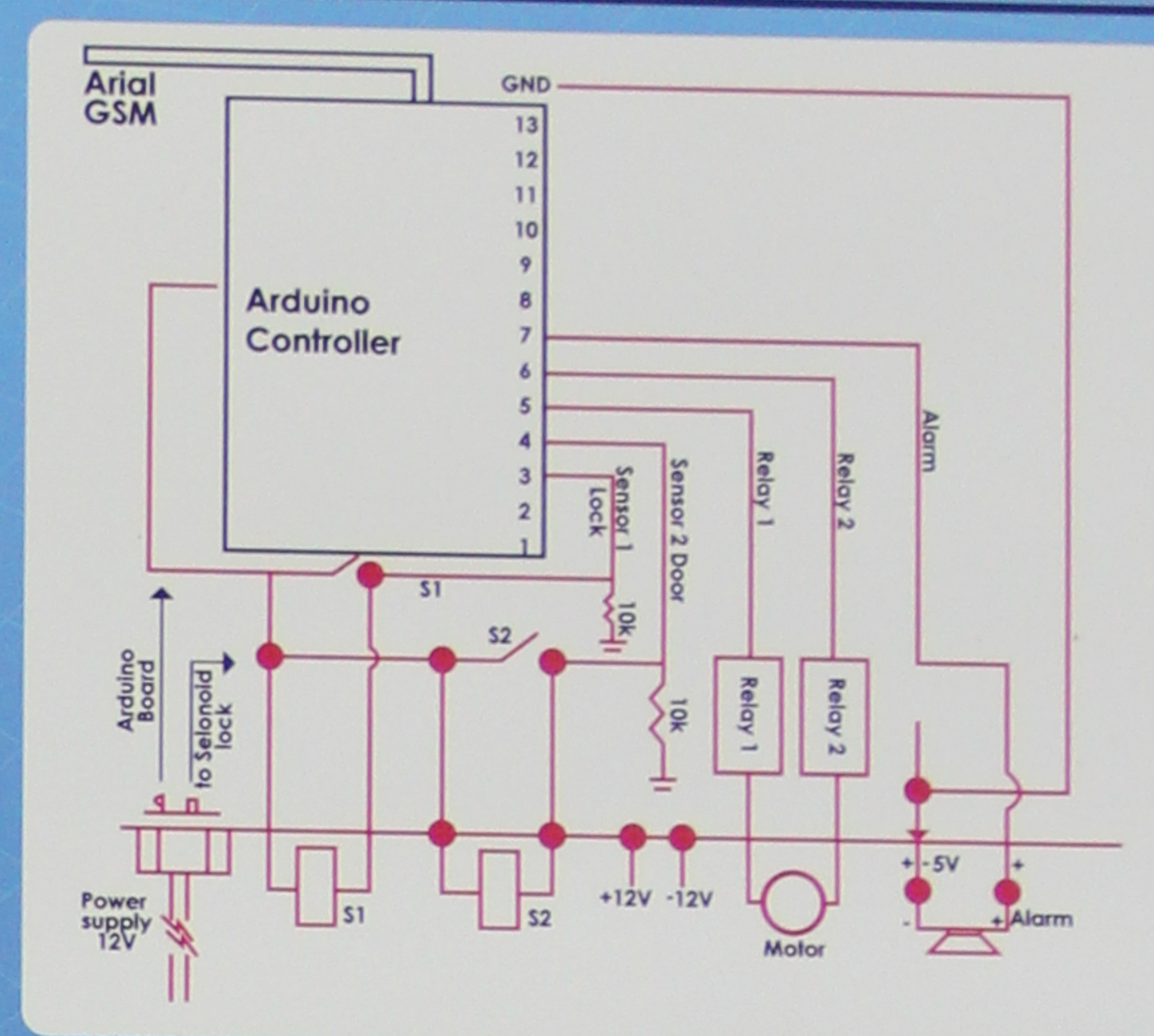
ARL Door System Circuit Diagram with GSM
