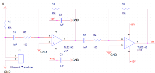
Figure 5 Signal conditioning circuit
