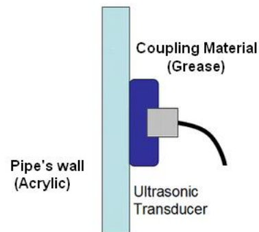
Figure 2 Acoustic coupling placement for ultrasound transmission
