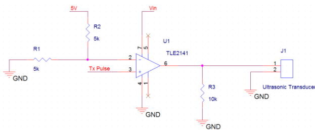
Figure 4 Pulse generator circuit schematic
