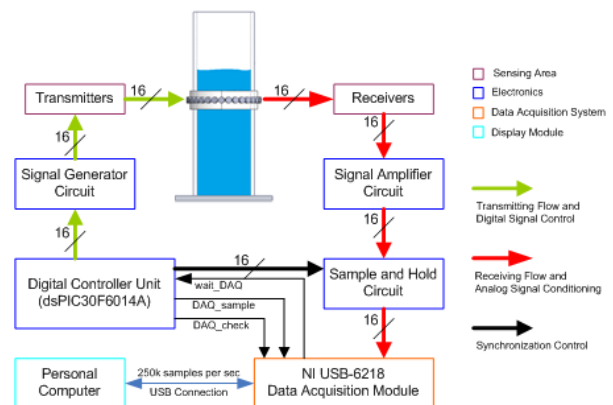
Figure 3 Electronics circuitry and the embedded system used in the Ultrasonic Tomography System
