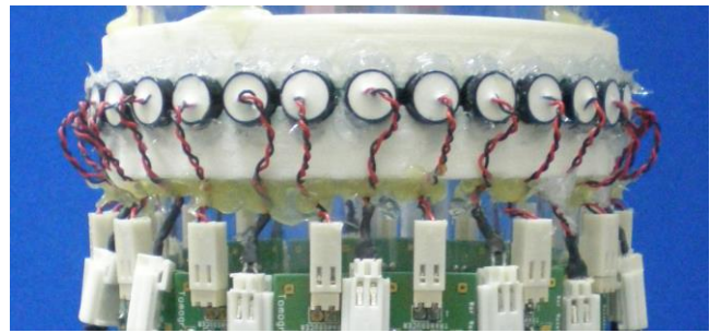
Figure 1 Sensing area consists of 16-pairs of ultrasonic transducers
