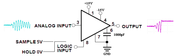
Figure 6 Typical sample and hold circuit
