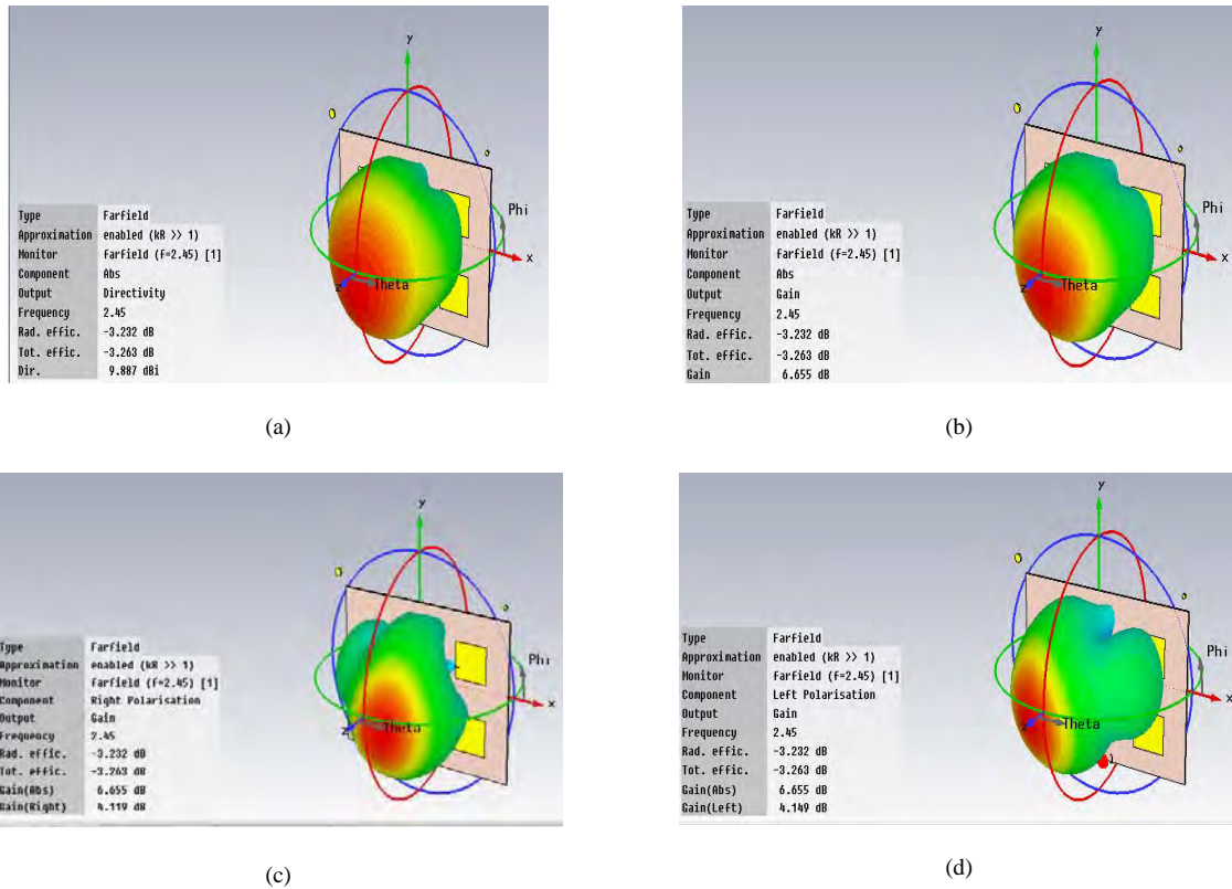
Figure 8: The simulated 3D Farfield radiation pattern of the proposed antenna
