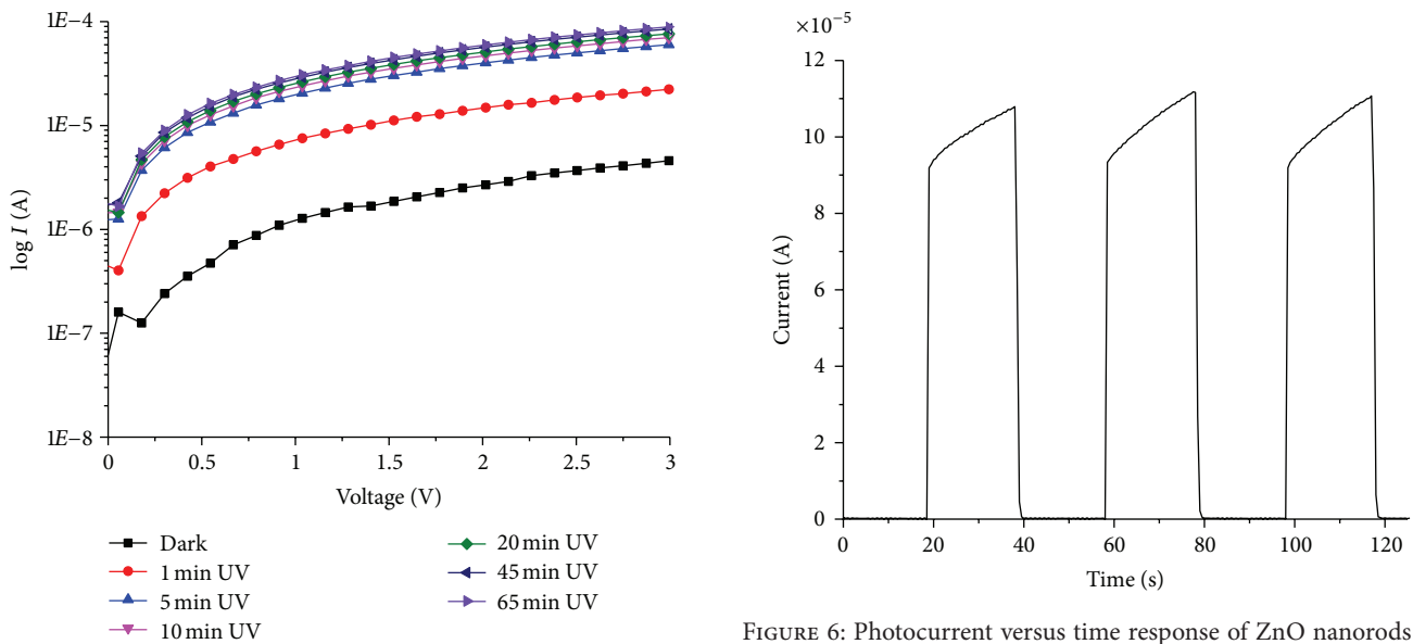
FIGURE 5: \log(I) versus voltage characteristic curves of ZnO nanorods.
