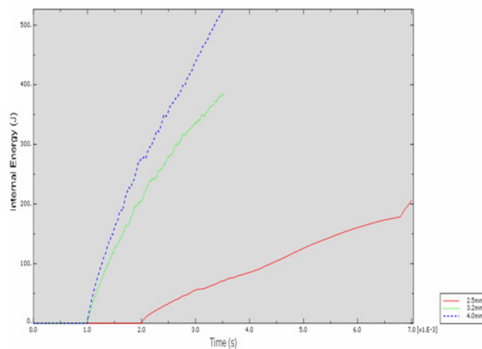
Figure 7: Energy absorbed for various wall thickness at constant speed 30m/s
