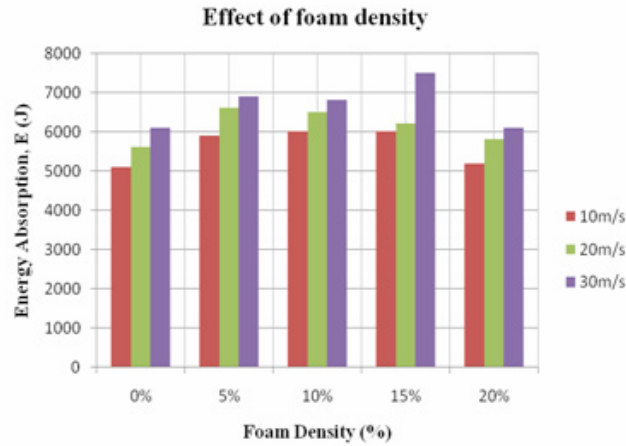
Figure 8: Energy absorption versus foam density
