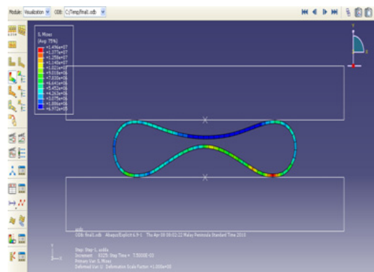
Figure 2: Collapse pattern of empty tube
