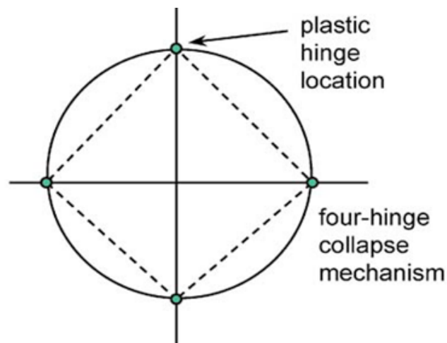
Figure 4: Four-hinge plastic mechanism
