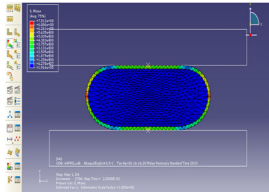
Figure 3: Collapse pattern of foam-filled Tube
