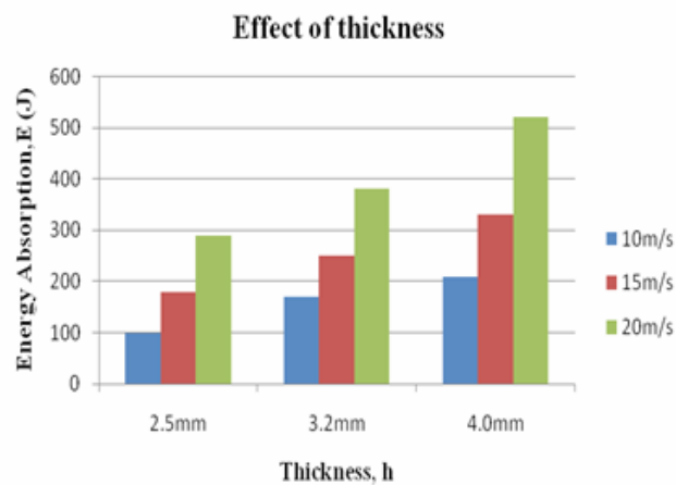
Figure 6: Energy absorption versus thickness for an empty cylindrical model
