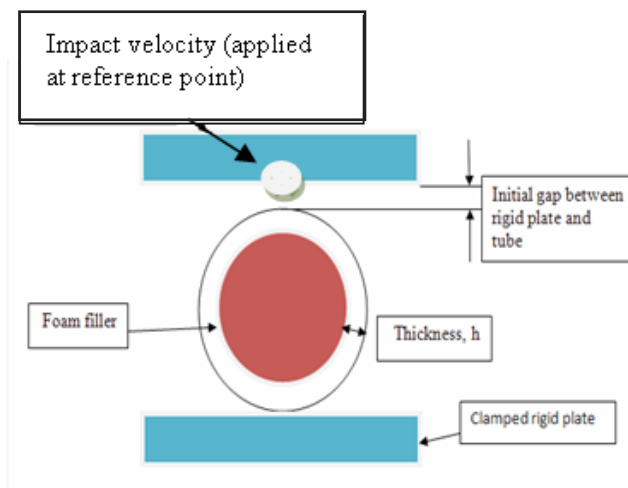
Figure 1: Cross-section of Numerical Model
