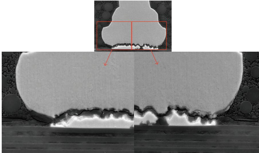
FIGURE 5: Typical AuAl IMC microcracks post extended HAST stress (1553 hr).
