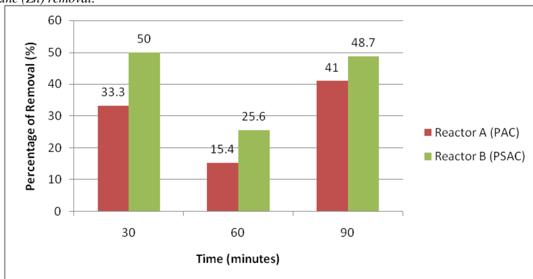
Fig. 3: Removal efficiency of zinc by Reactor A and B.
