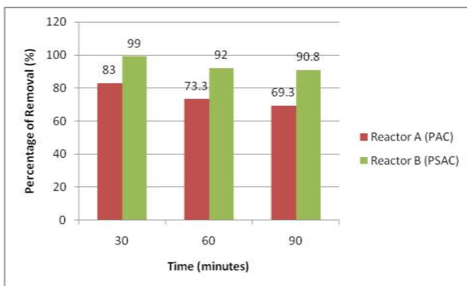
Fig. 2: Removal efficiency of iron by Reactor A and B.
