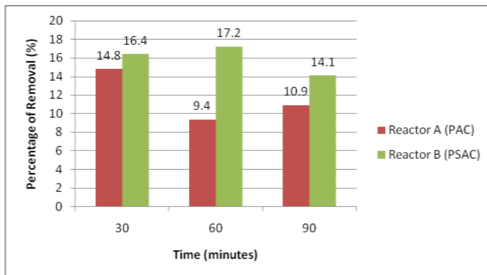
Fig. 1: Removal efficiency of copper by Reactor A and B.
