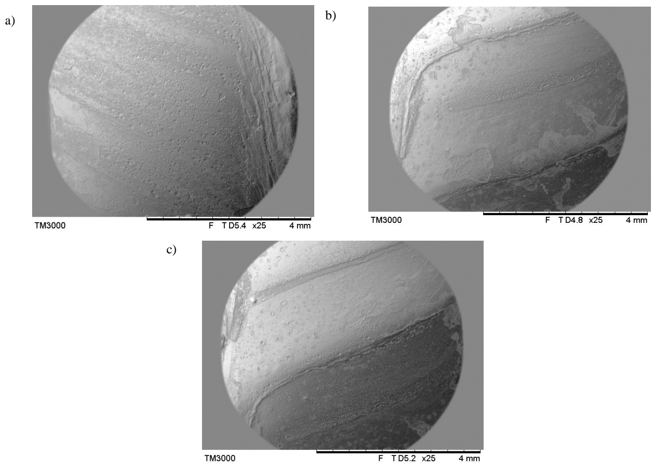
a) MRR = 5500-6400 \text{ mm}^3/\text{min} , SR = 20-30 \text{ }\mu\text{m} b) MRR = 3600-4800 \text{ mm}^3/\text{min} , SR = 30-50 \text{ }\mu\text{m} c) MRR = 3000-3500 \text{ mm}^3/\text{min} , SR = 65-80 \text{ }\mu\text{m}
