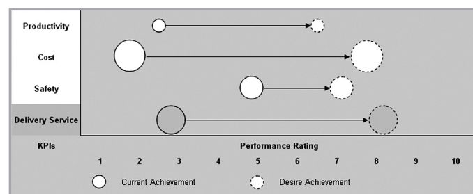
Figure 1: Gap analysis
