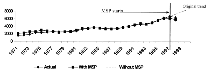
Figure 8: Predictive Model of yearly Traffic Deaths
