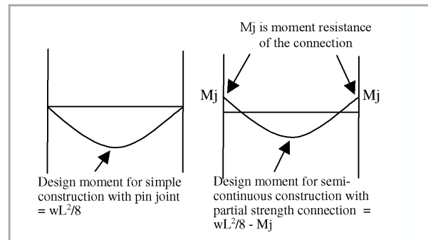
Figure 2: Design moment for beams due to different support conditions
